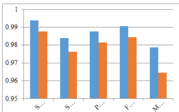
Fig 5. Performance measures
